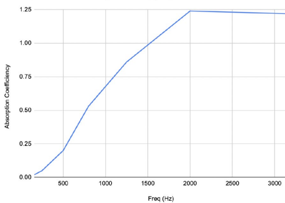
Absorption Coefficient vs. Freq (Hz)
